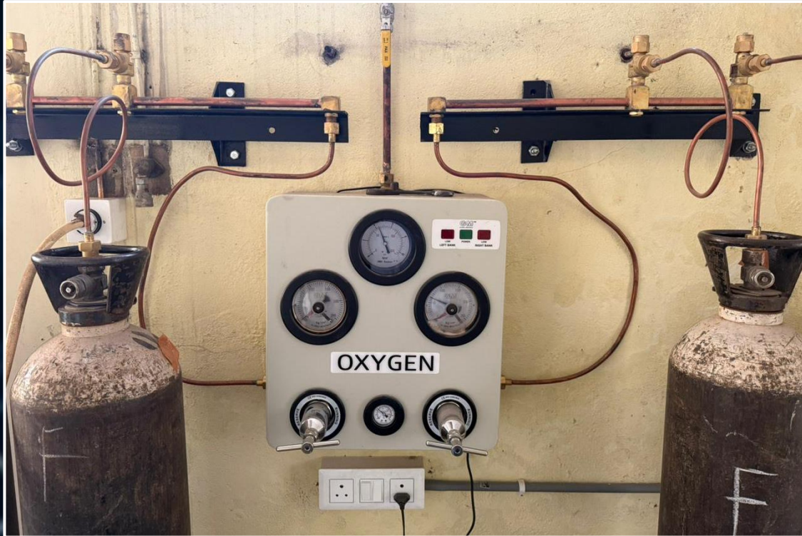
SEMI AUTOMATIC OXYGEN CONTROL PANEL FOR MANIFOLD ROOM
